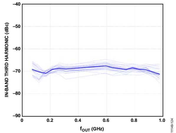
Figure 113. Third Harmonic vs. f_{OUT} Performance for Eight DOCSIS Carriers
