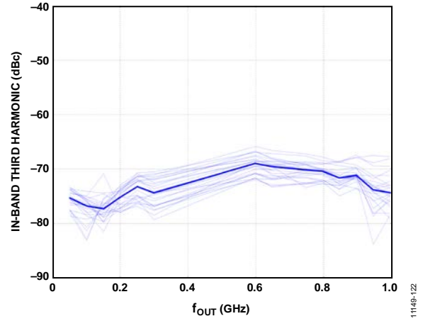
Figure 111. Third Harmonic vs. f_{OUT} Performance for One DOCSIS Carrier
