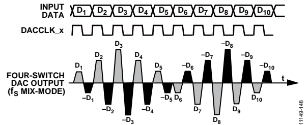
Figure 145. Mix-Mode Waveform
