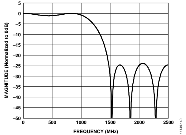
Figure 137. FIR25 2\times Interpolation Filter Plot, Complete Frequency Response; f_{DAC} = 2.5 GHz
