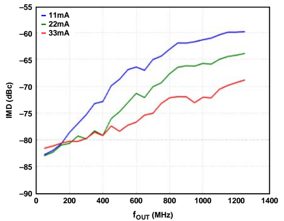
Figure 73. IMD vs. f_{OUT} over DAC I_{OUTFS}
