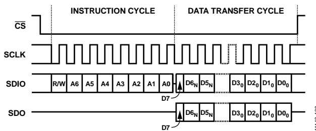
Figure 123. Serial Register Interface Timing, MSB-First Read
