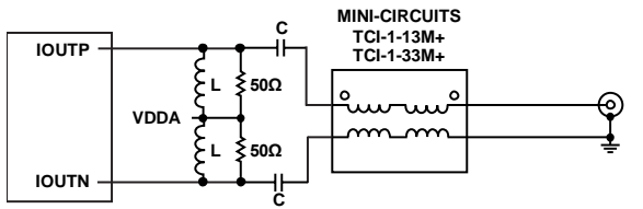
Figure 154. Recommended Mix-Mode Configuration Offering Extended RF Bandwidth Using TCI-1-13M+ Balun
