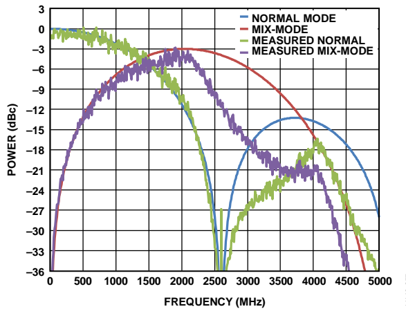
Figure 155. Measured vs. Ideal DAC Output Response; f_{DAC} = 2.6 GSPS
