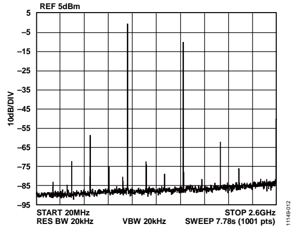
Figure 13. Single-Tone Spectrum at f_{OUT} = 1000 \text{ MHz}
