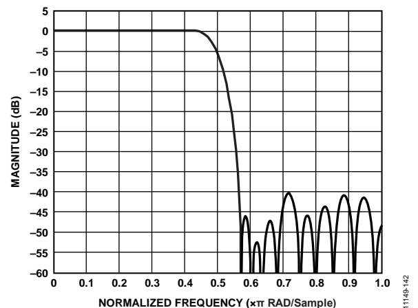
Figure 139. FIR40 2\times Interpolation Filter Plot, Complete Frequency Response
