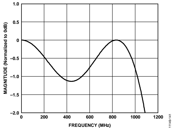
Figure 138. FIR25 2\times Interpolation Filter Plot, Pass-Band Ripple; f_{DAC} = 2.5 GHz
