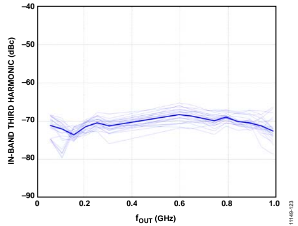
Figure 112. Third Harmonic vs. f_{OUT} Performance for Four DOCSIS Carriers
