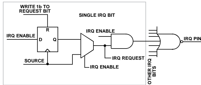
Figure 141. Interrupt Request Circuitry
