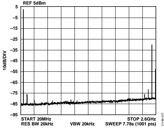
Figure 62. Single-Tone Spectrum at f_{OUT} = 70 \text{ MHz}
