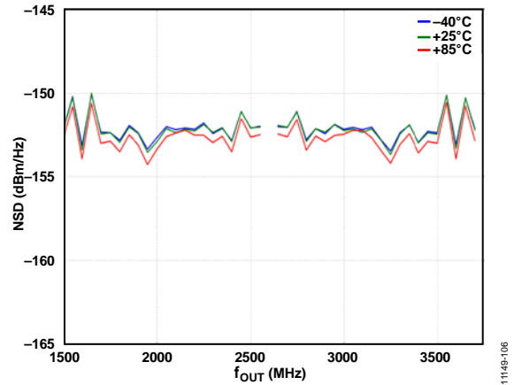
Figure 96. W-CDMA NSD vs. f_{OUT} over Temperature
