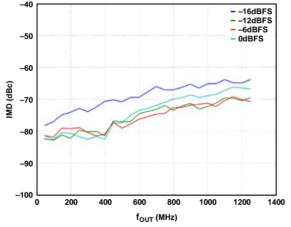
Figure 71. IMD vs. f_{OUT} over Digital Full Scale
