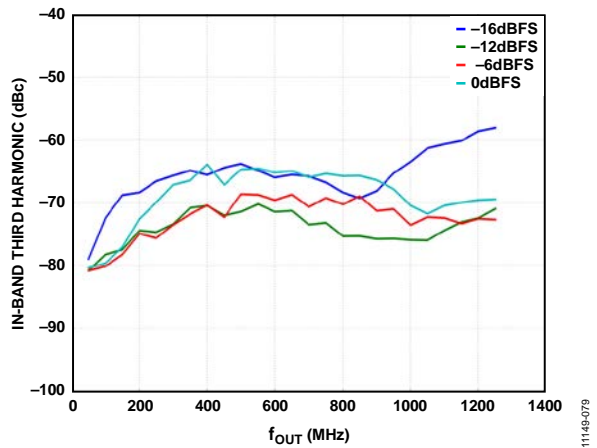
Figure 70. SFDR for Third Harmonic vs. f_{OUT} over Digital Full Scale
